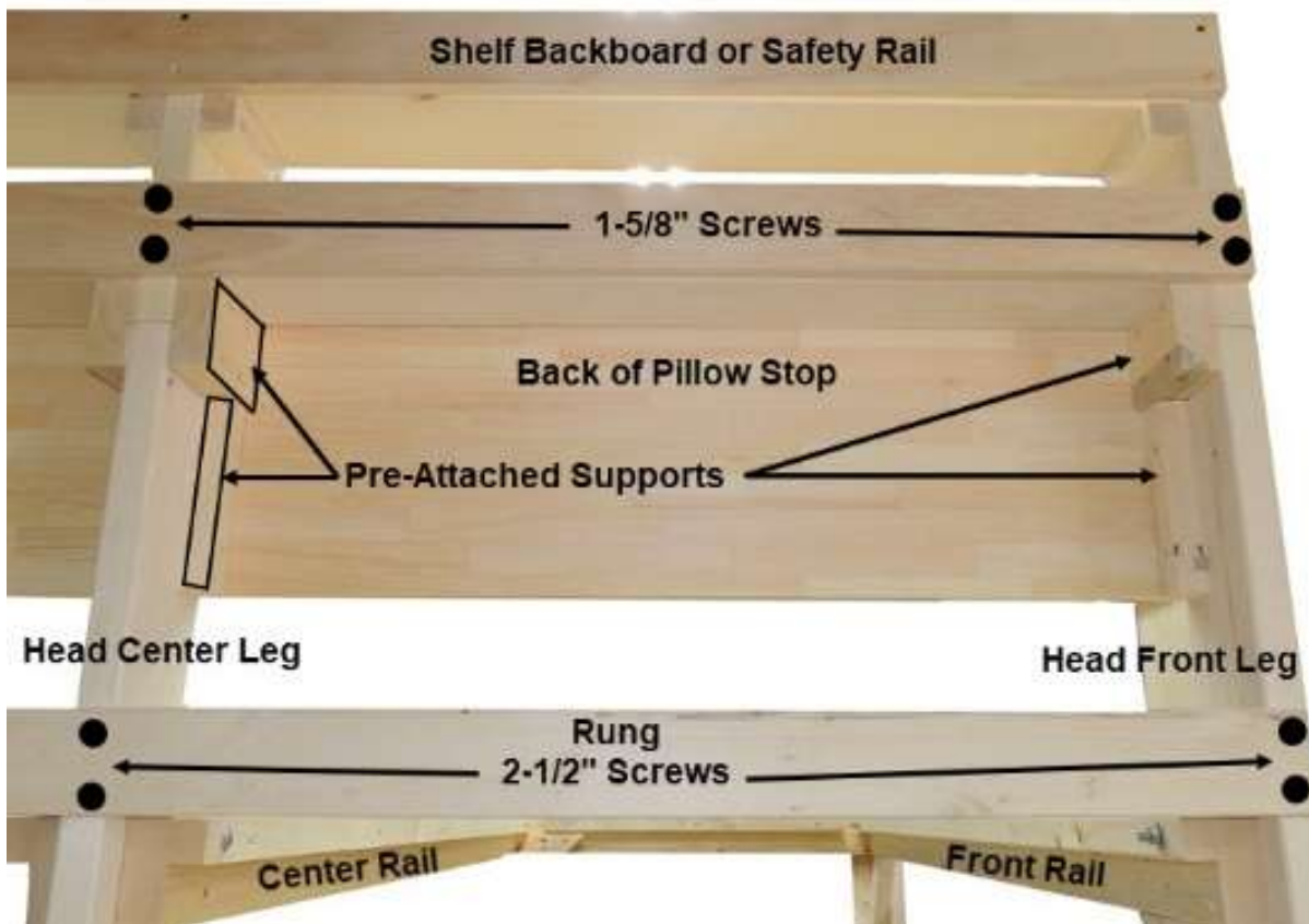
Pillow Stop Back View
