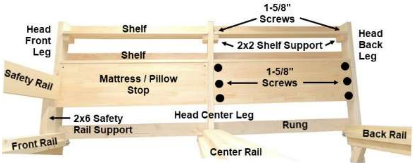
Pillow Stop Front View
